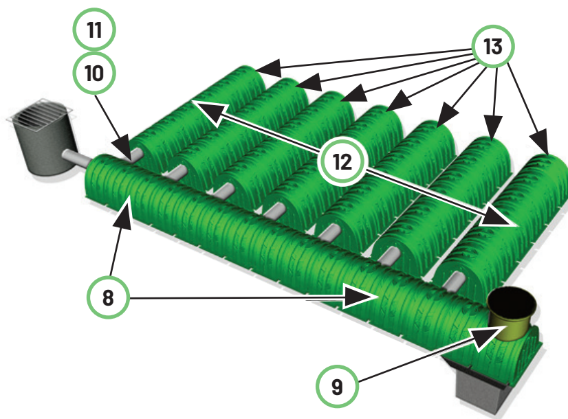
FIGURE 3 - Distribution Pipes
